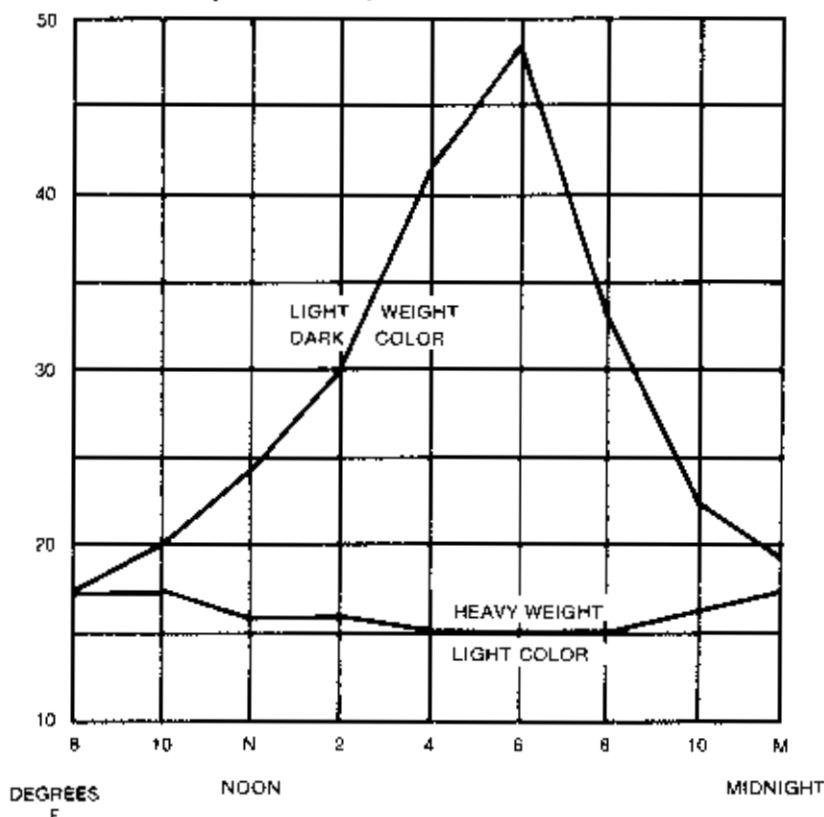
Total Equivalent Temperature Differentials—West Wall
