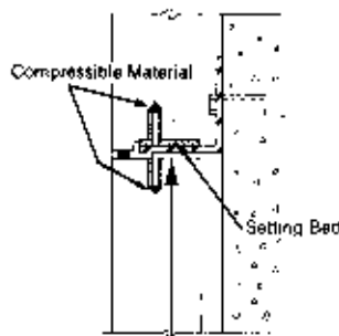
OPEN SPACE UNDER ANGLE
