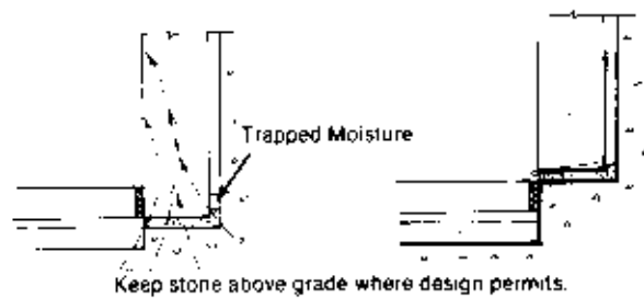
Keep stone above grade where design permits.
