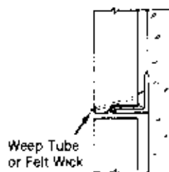
Weep continuous and other angle supports where moisture collects
