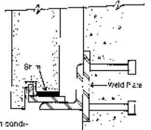
Lateral Adjusting Plate with S.S. Bar, Field Weld Plate to Angle
