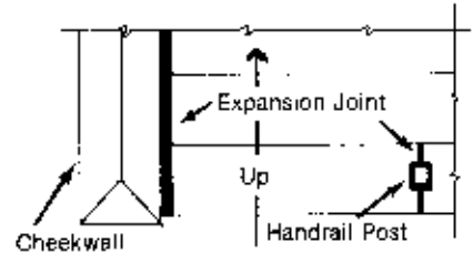
EXPANSION JOINT AT STAIR ENDS AND HANDRAIL POSTS
