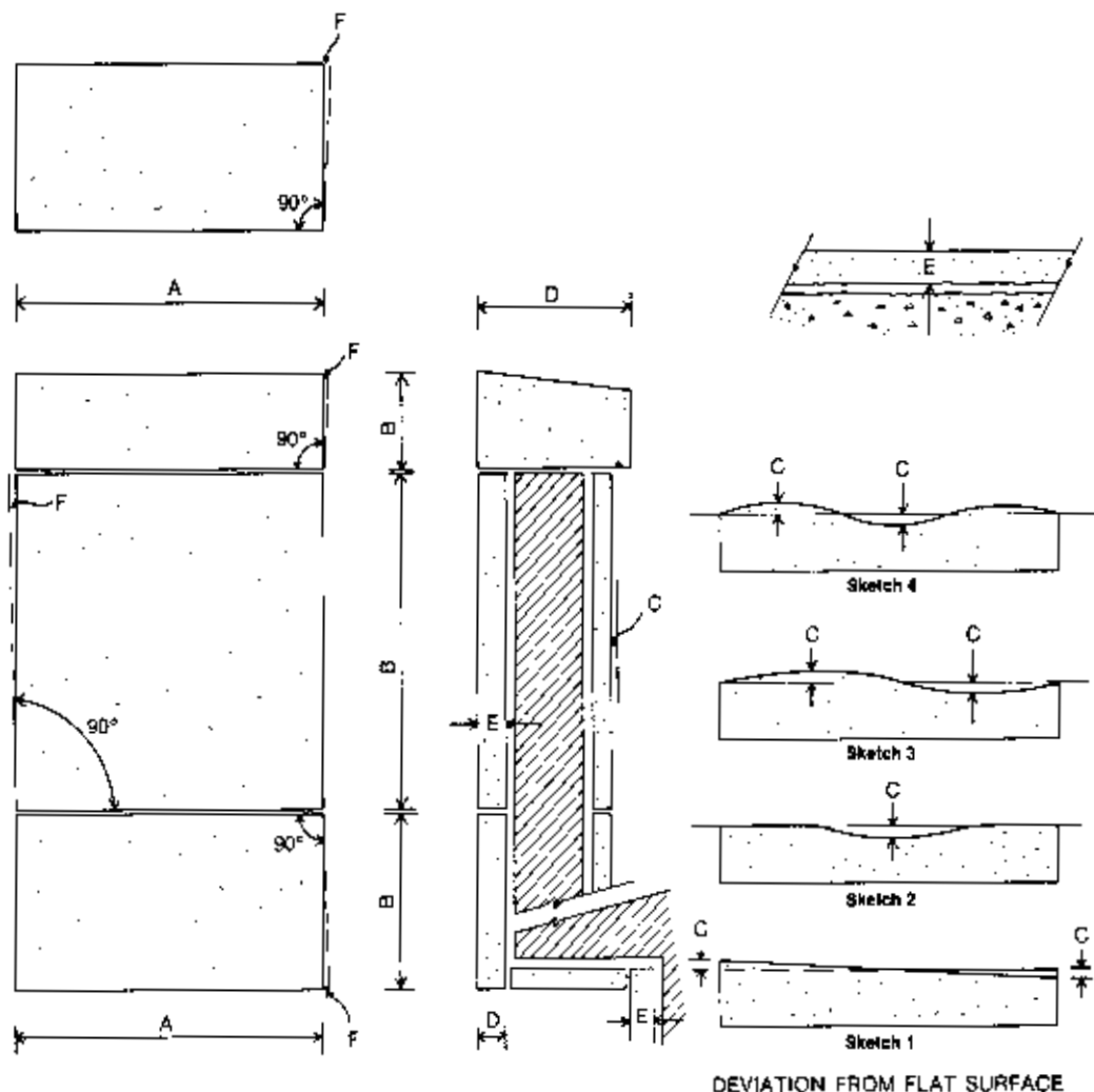
DEVIATION FROM FLAT SURFACE
