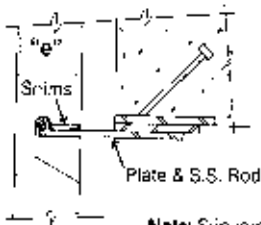
Isometric of Typical Angle with Lateral Adjusting Plates & S.S. Bars, Field Weld Plate to Angle
